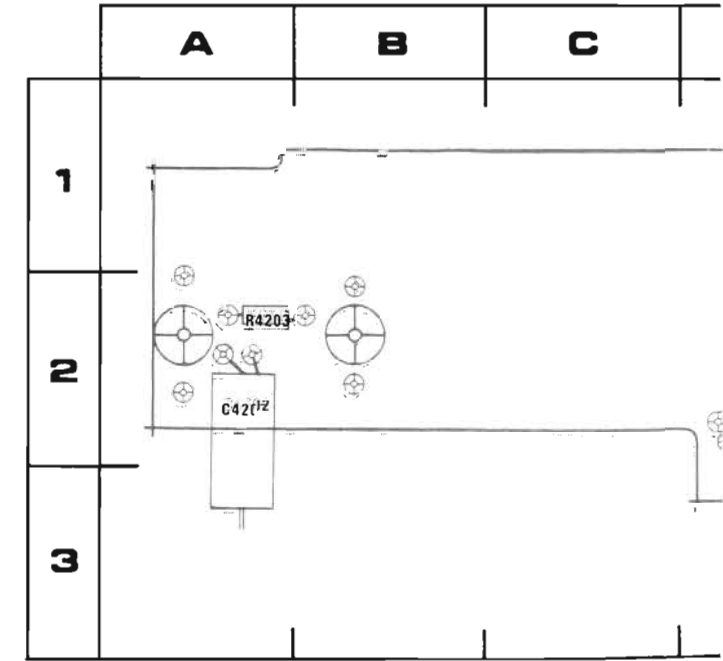
E. A3 CAM SWITCHING BOARD (BOTTOM).
