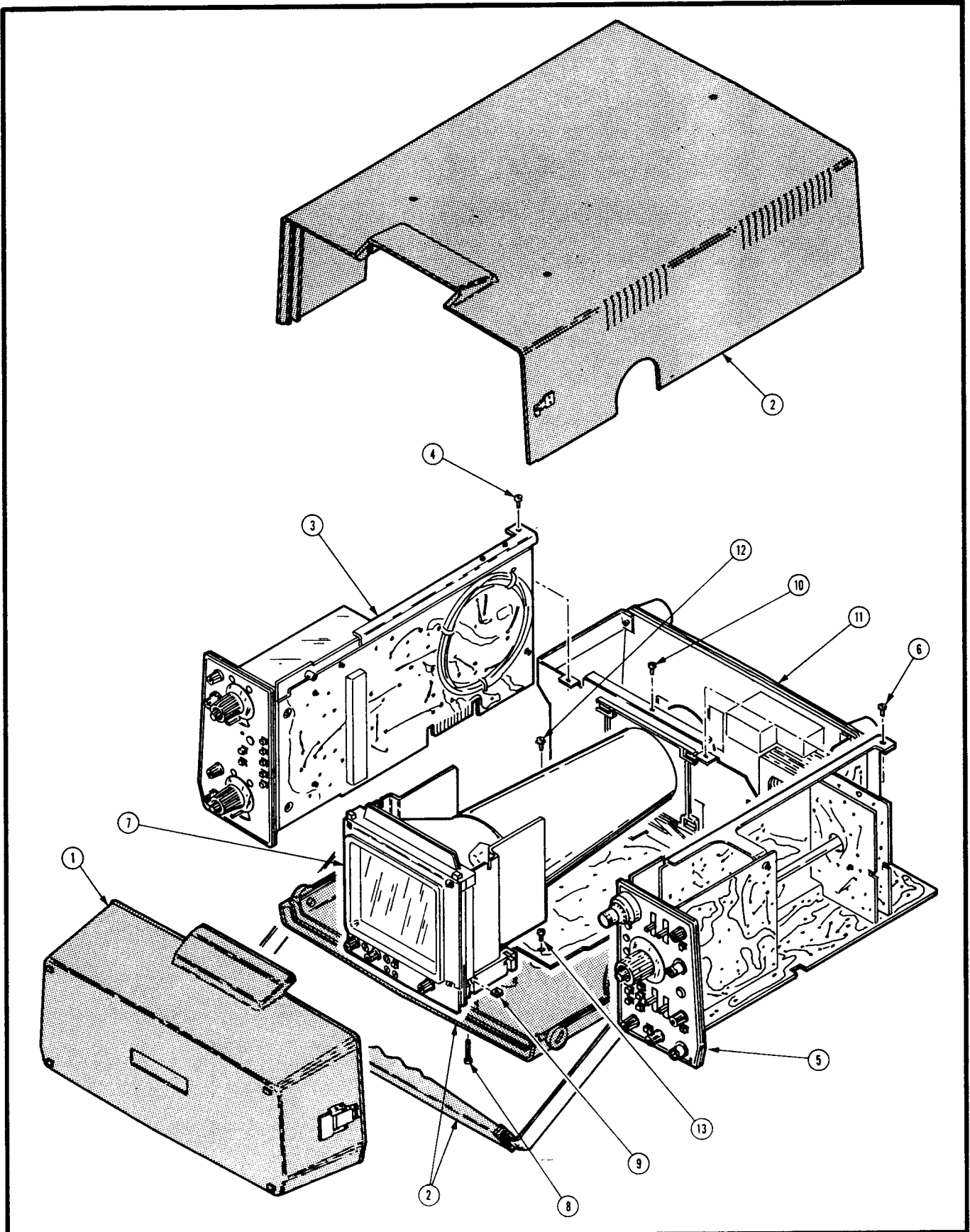
Figure 8-1. Oscilloscope, AN/USM-425(V)1.
