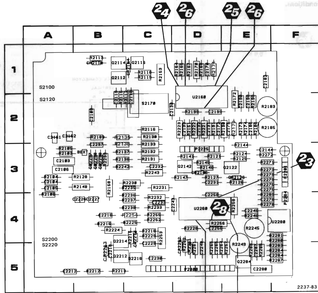
B. A7 TRIGGER BOARD
