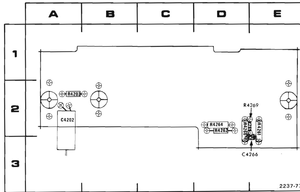
E. A3 CAM SWITCHING BOARD (BOTTOM).
