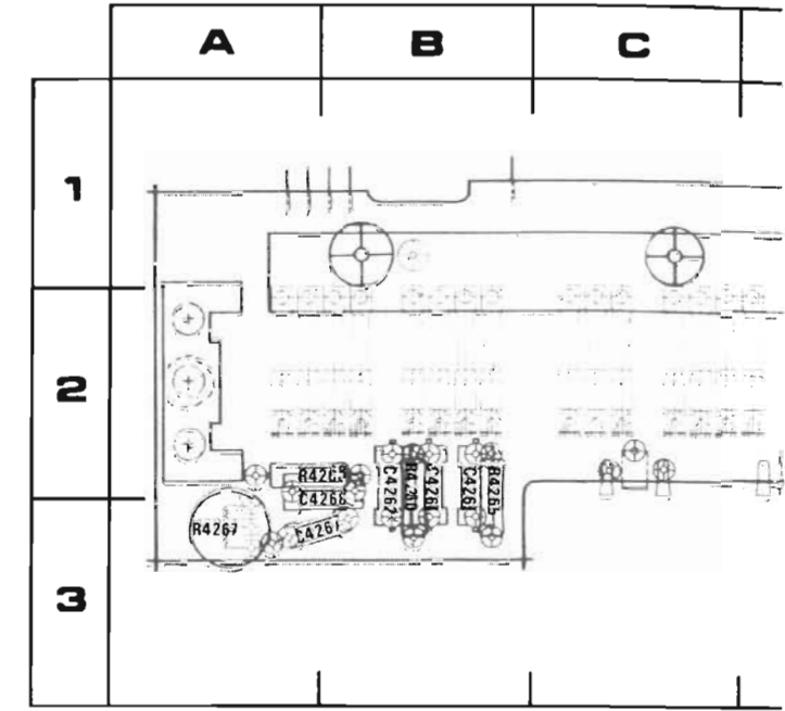
D. A3 CAM SWITCHING BOARD (TOP).
