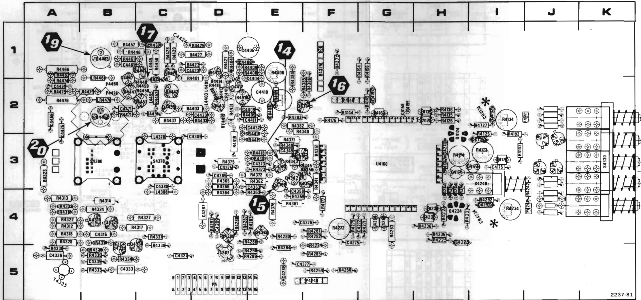
FO-3 (Rear). A5 Vertical circuit board layout and component locator.
