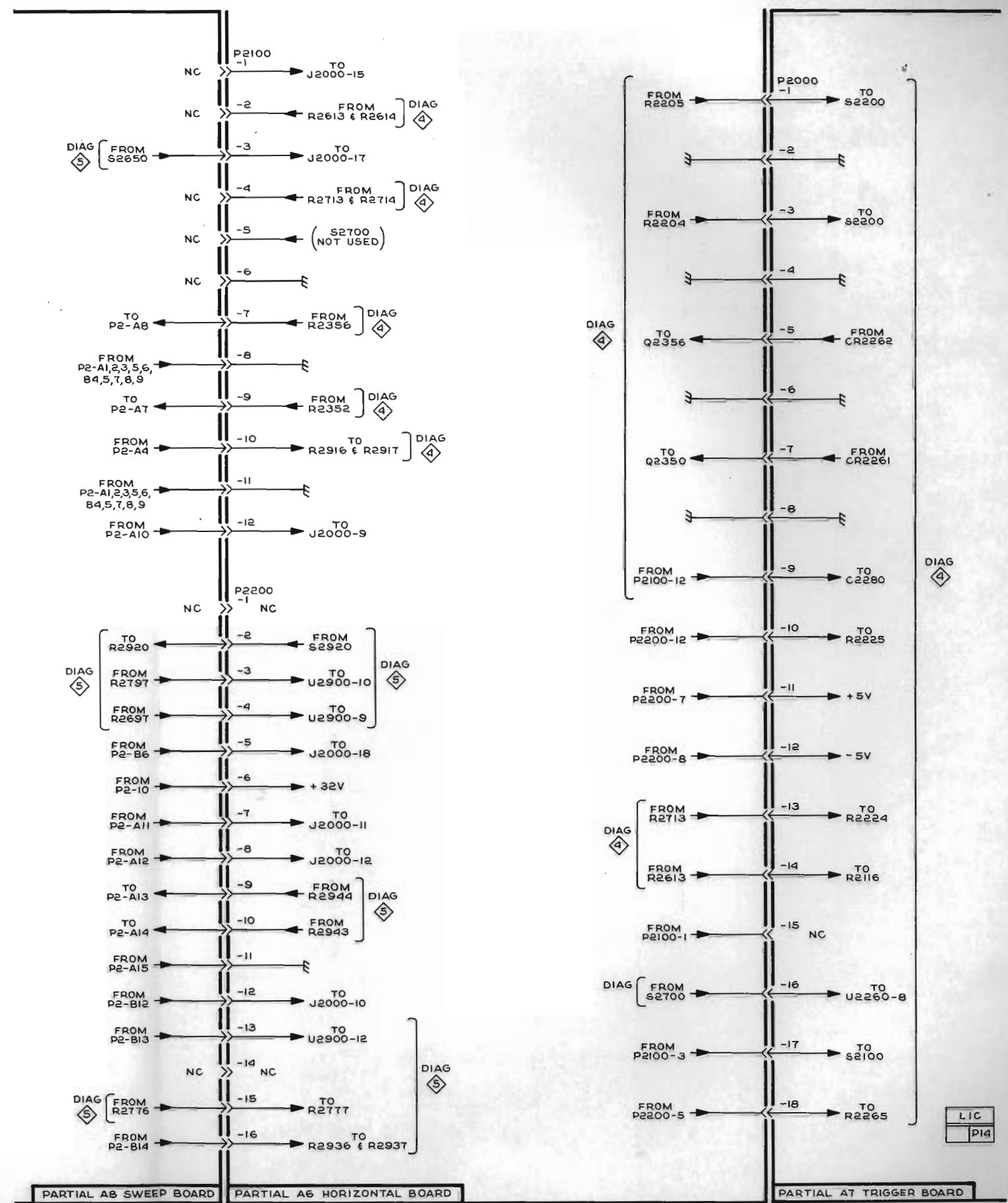
Figure FO-11 (Front). Interconnect Wiring schematic diagram.
