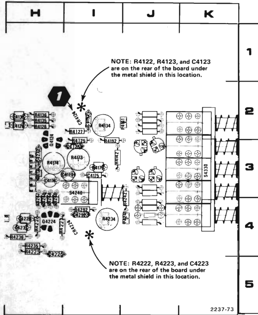
A. PARTIAL AS VERTICAL BOARD.
