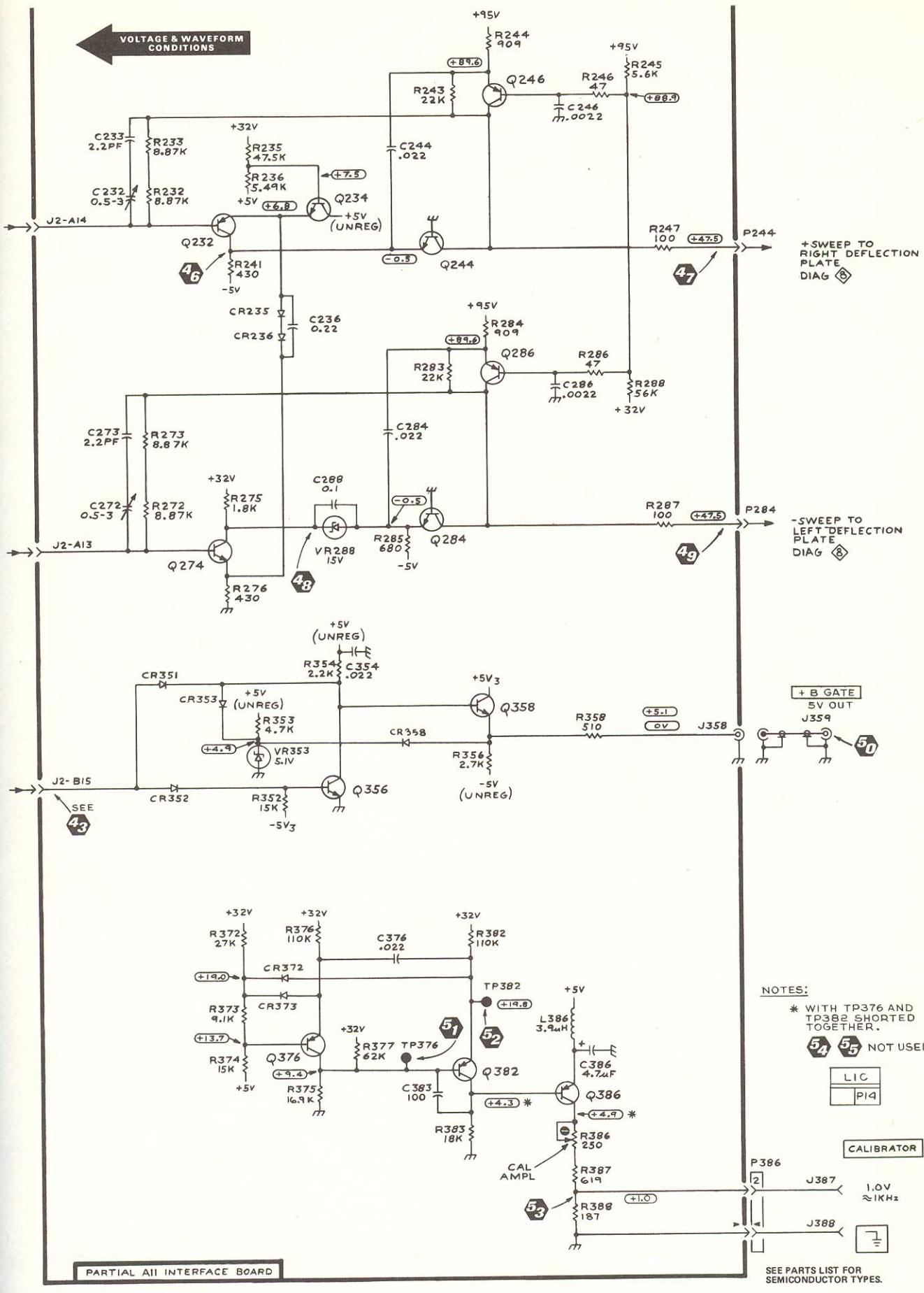
Figure FO-8 (Front). Horizontal Amplifier, + Gate, and Calibrator schematic diagram.
