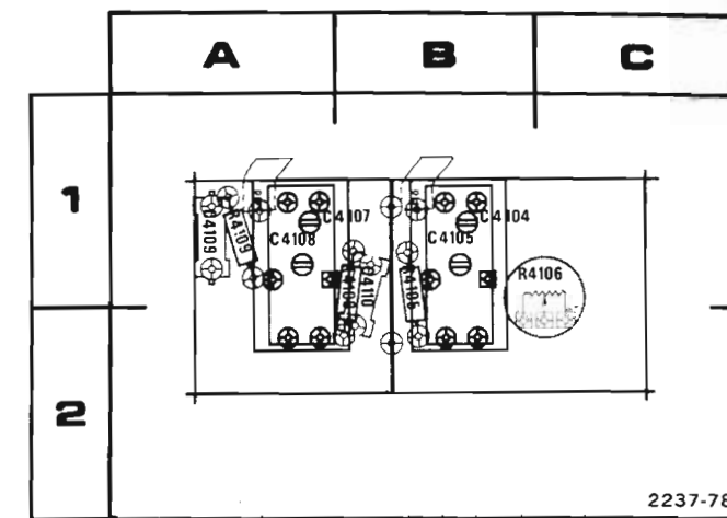
F. A2 ATTENUATOR BOARD.
