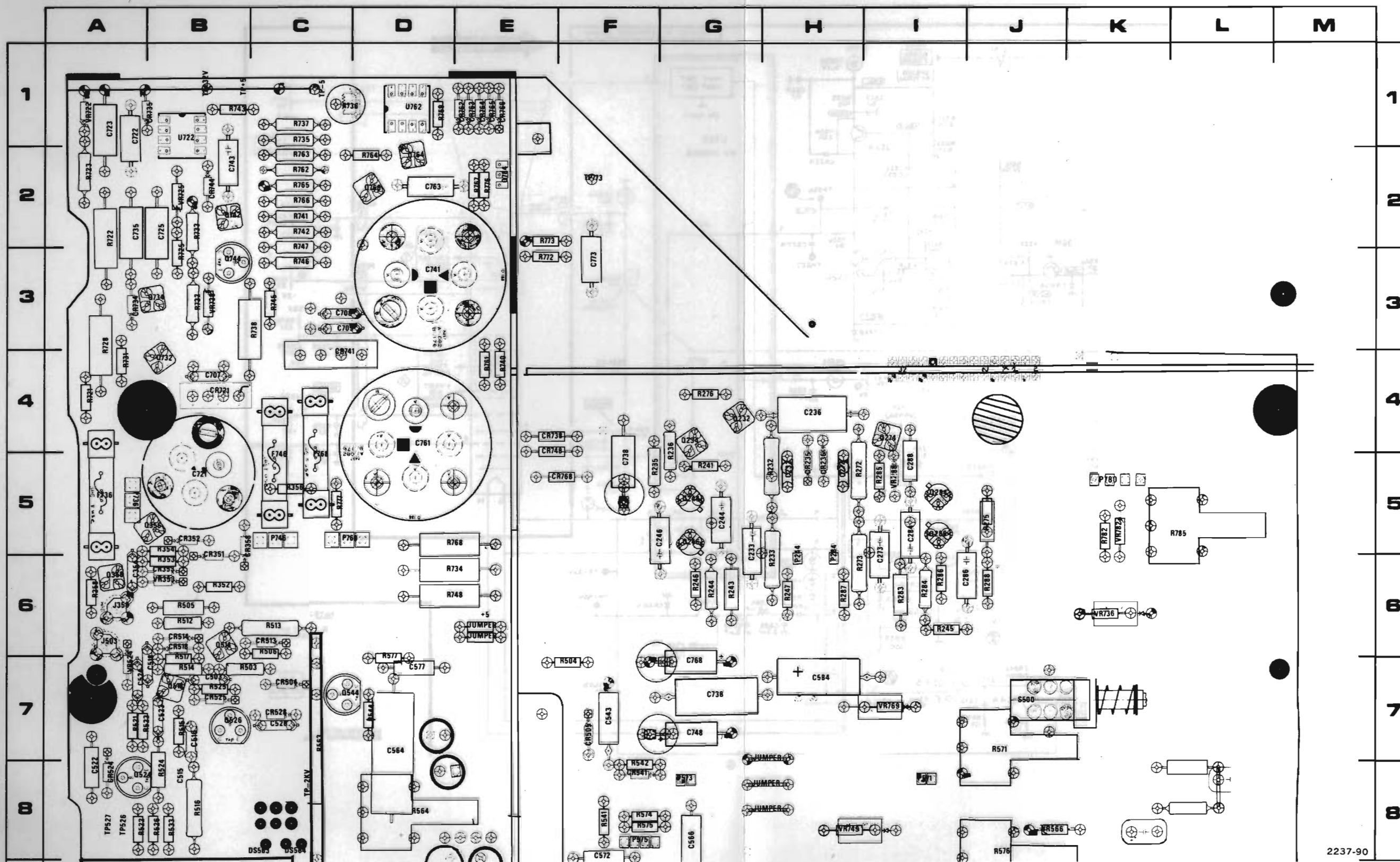
Figure FO-9 (Rear). Partial A11 Interface circuit board layout and component locator.
