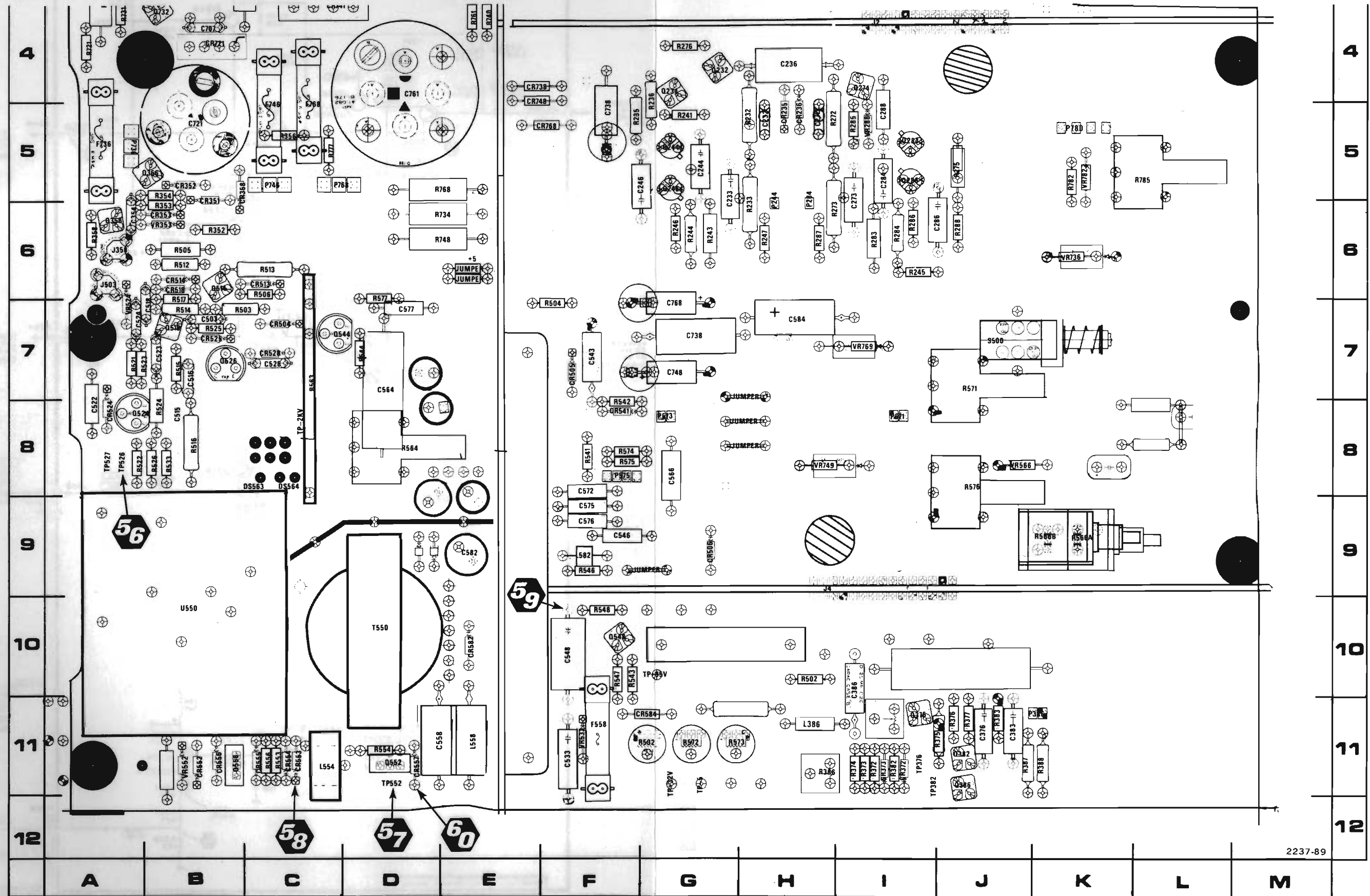
Figure FO-8 (Rear). Partial A11 Interface circuit board layout and component locator.
