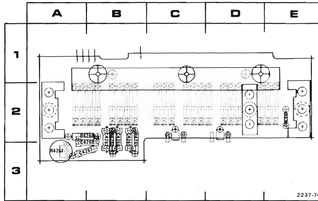
D. A3 CAM SWITCHING BOARD (TOP).
