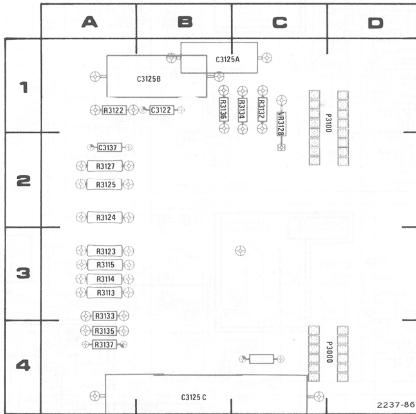
A. A9 A TIMING SWITCH BOARD.
