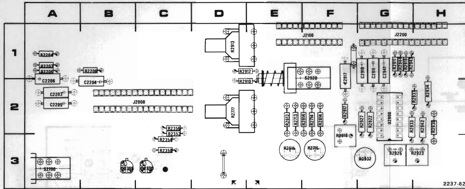
A. A6 HORIZONTAL BOARD.
