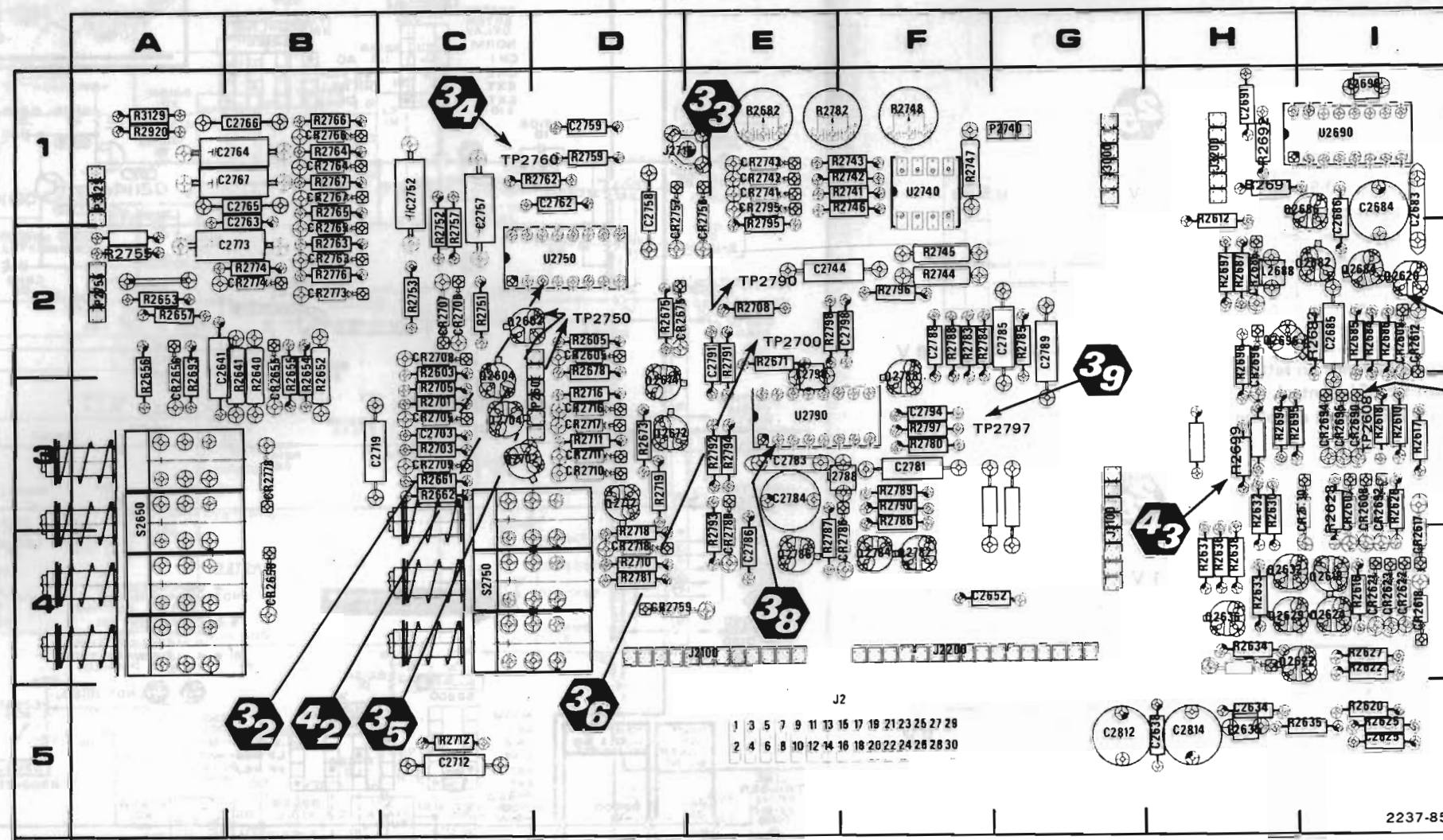
B. A8 SWEEP BOARD.
