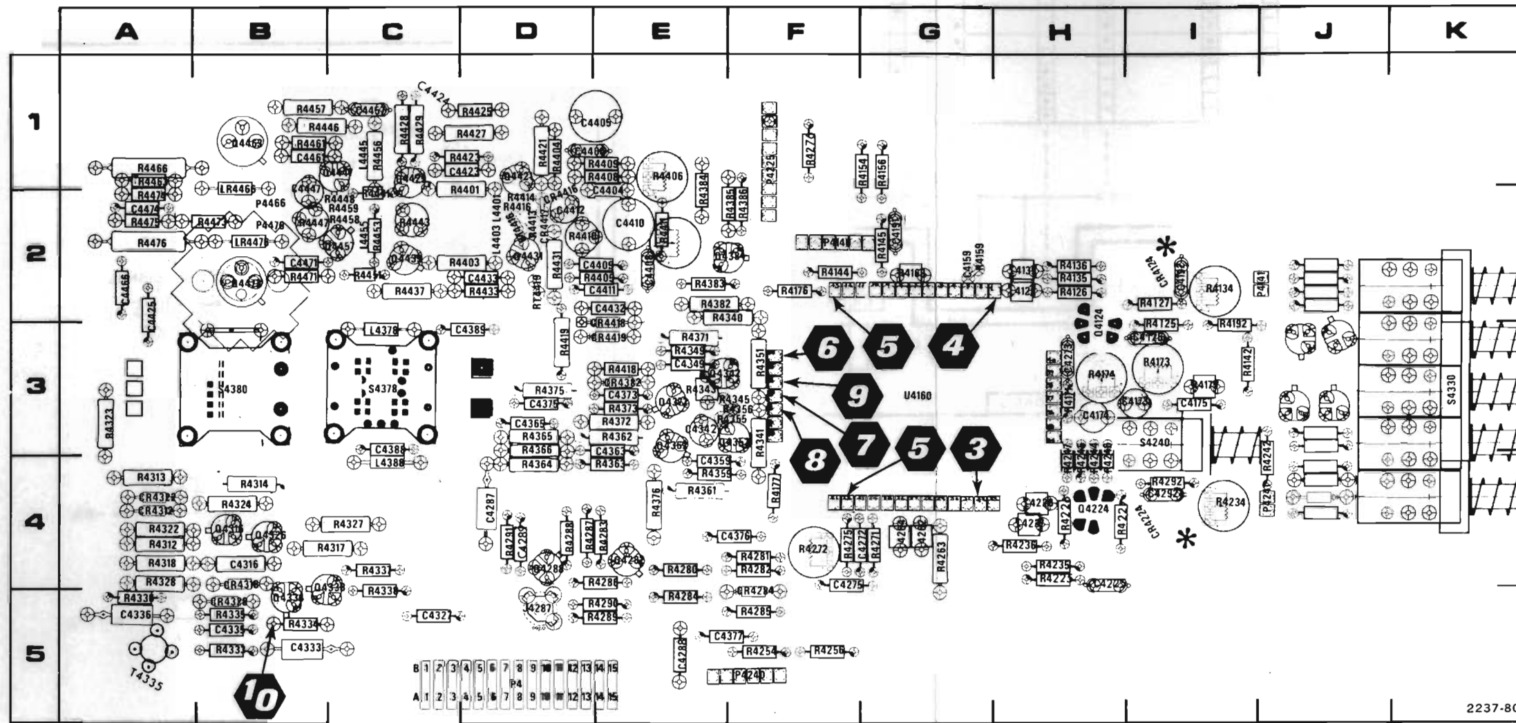
Figure FO-2 (Rear). A5 Vertical circuit board layout and component locator.
